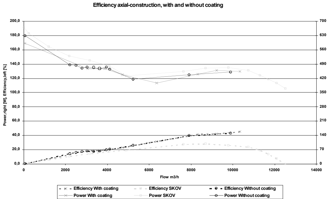
Figure 8: Efficiency, small ventilator
