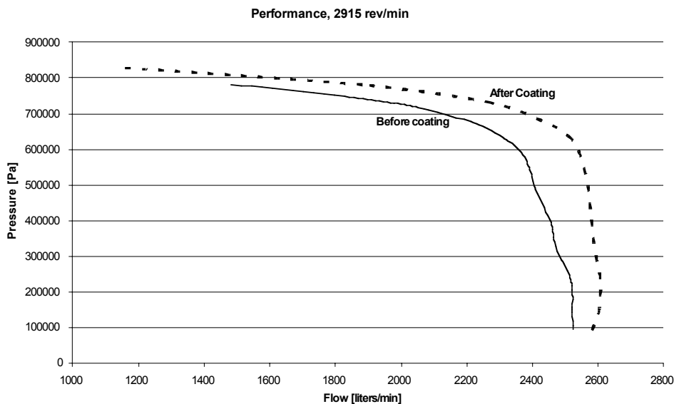
Figure 1. Pump performance, high pressure used pump / paper mill
