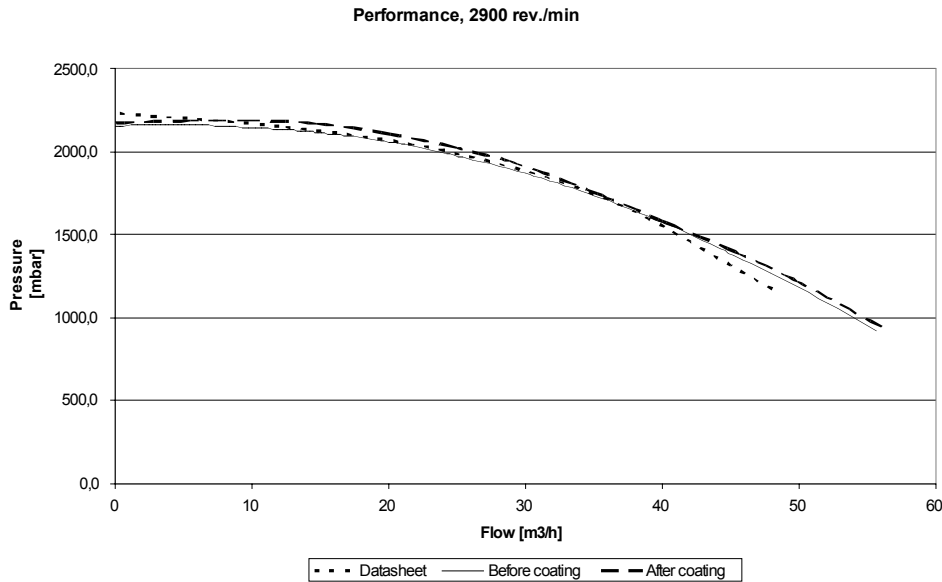
Figure 5. Pump performance, small low pressure new pump
