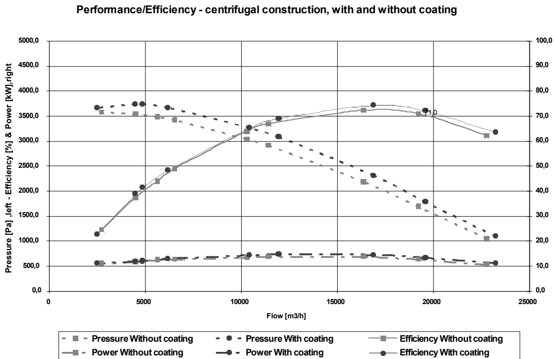
Figure 9: Performance & Efficiency, medium sized ventilator
