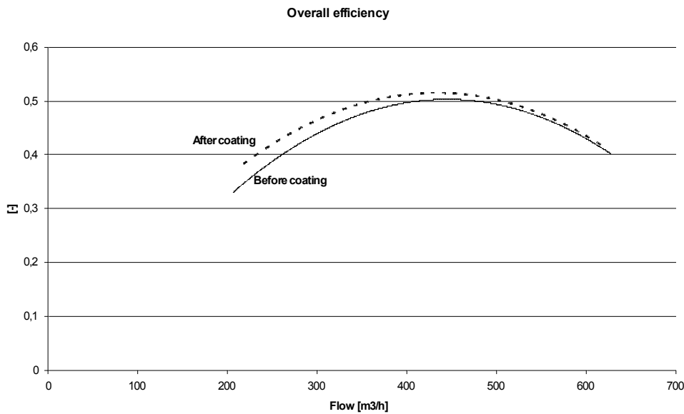
Figure 4. Overall efficiency, low pressure used pump (renovated) / waste water
