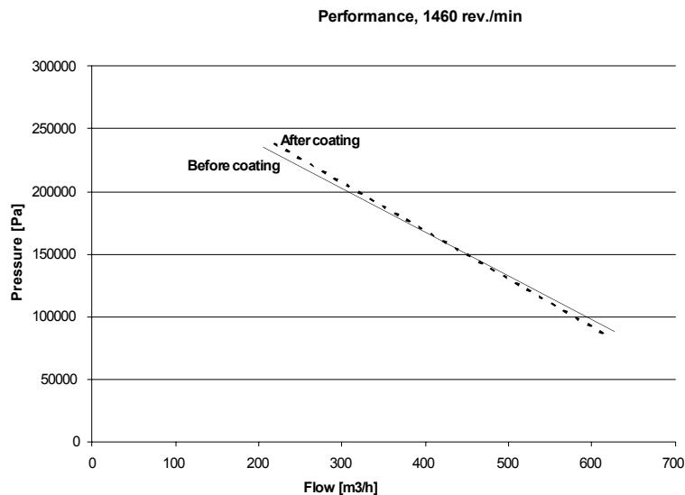
Figure 3. Pump performance, low pressure used pump / waste water
