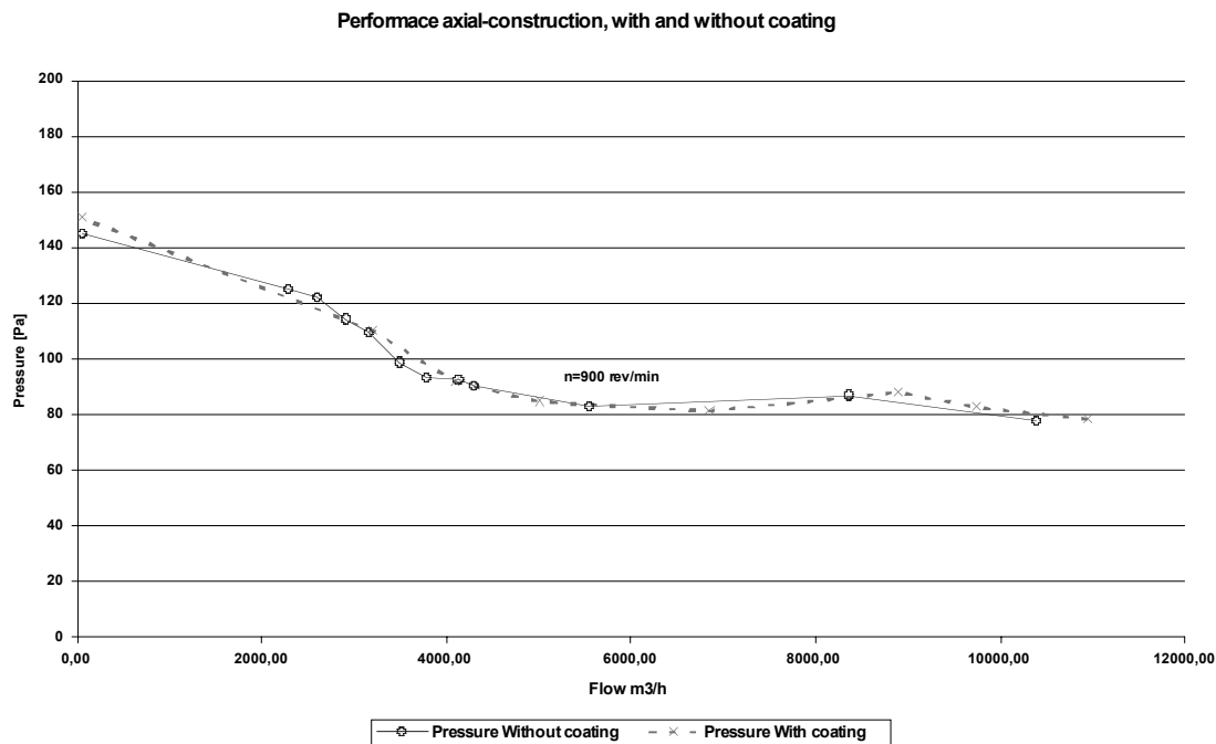
Figure 7: Performance, small ventilator
