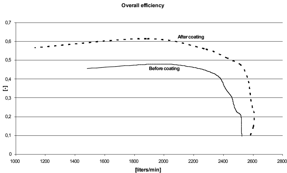
Figure 2. Overall efficiency, high pressure used pump / paper mill
