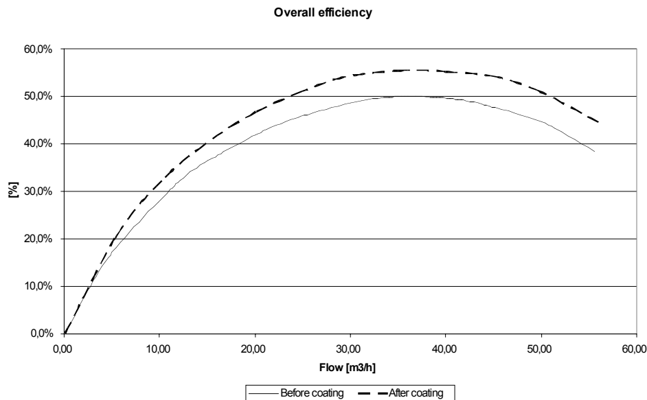
Figure 6: Overall efficiency, small low pressure new pump
